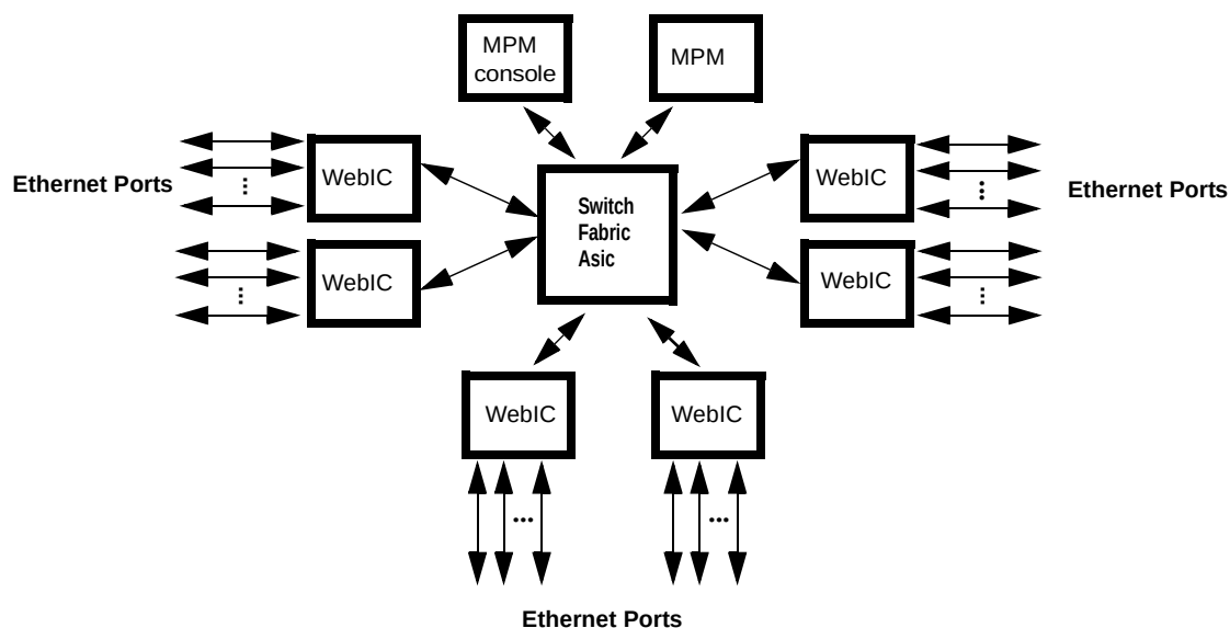
Figure 2 Basic Architecture of WebIC ASIC–Switch Fabric ASIC
