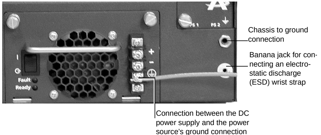
Figure 10 Attaching DC Power to the Power Supply Terminals
