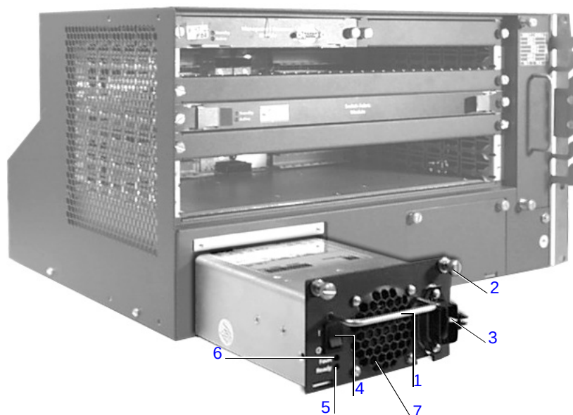
Figure 9 Power Supply Faceplate
