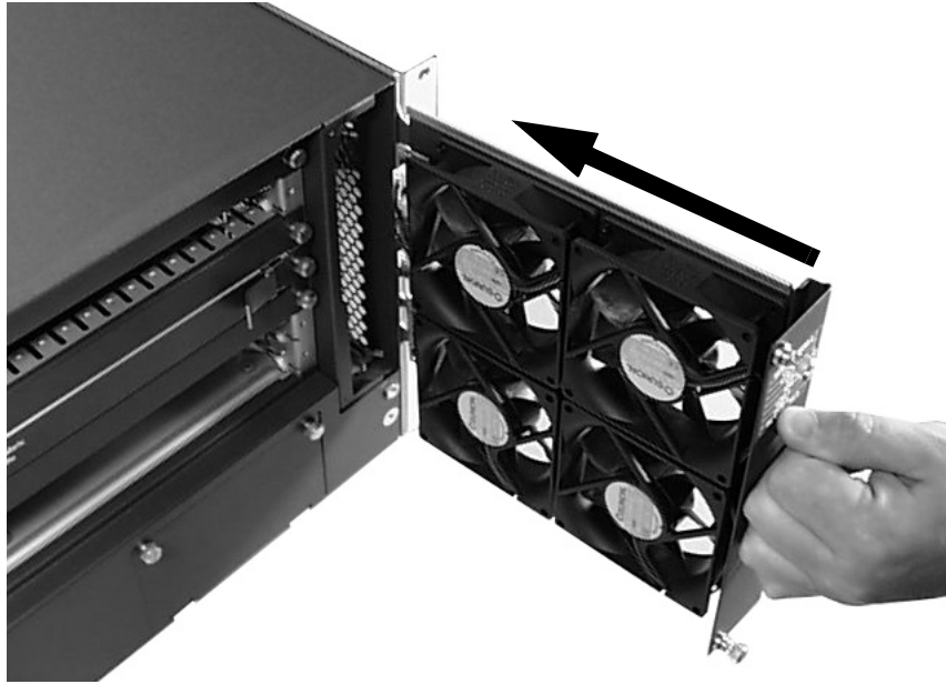
Figure 26 Inserting the Fan Tray
