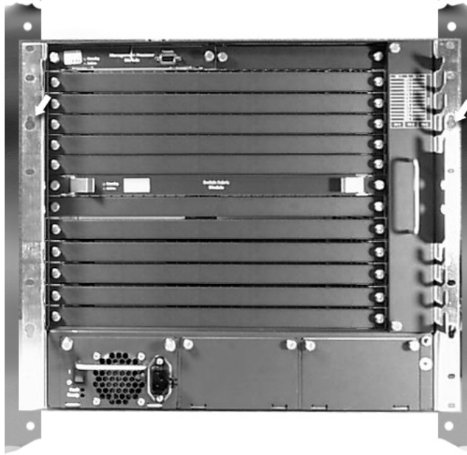
Figure 7 Installing Guide Screws in the Rack Frame
